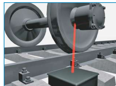
Positioning in hot box detection systems
